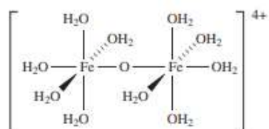
Slika 13. Struktura [(\text{H}_2\text{O})_5\text{FeOFe}(\text{H}_2\text{O})_5]^{4+} .
