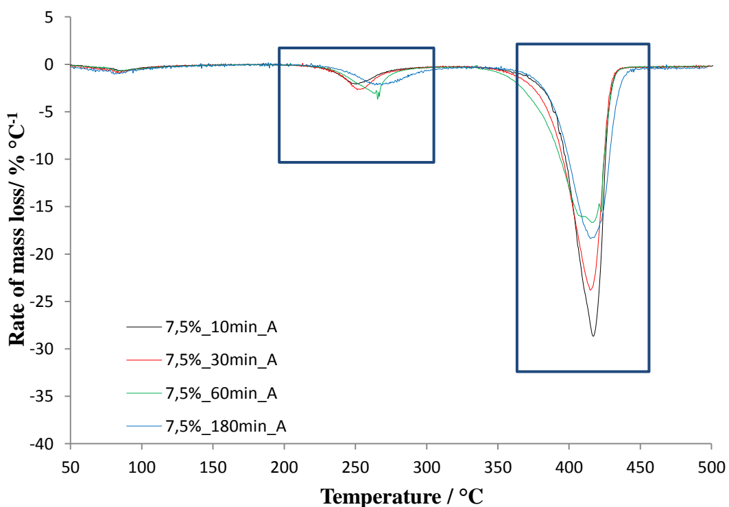
Figure 66. DTG curves of the nonisothermal degradation for the films after immersion in 7.5% w/v CaCl 2 solution for 10, 30, 60 and 180 min with single rinse (A)
