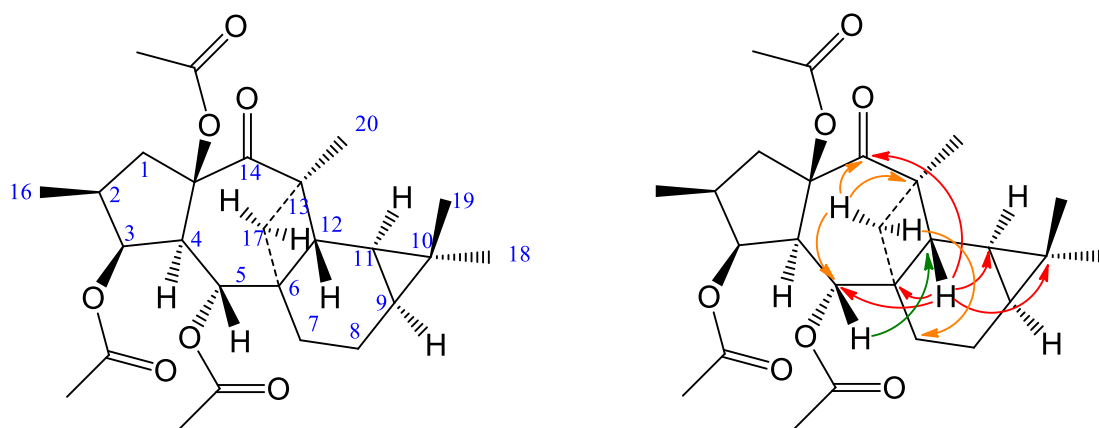
Figure 6. Selected HMBC correlations observed for compound 23
