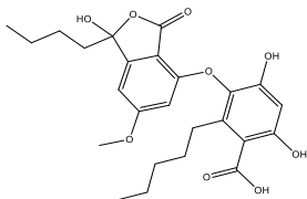
Lobarin
