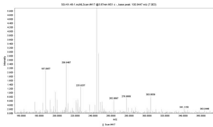
Figure S34. Mass spectrum of nonanedioic acid with m/z 187.0957.
