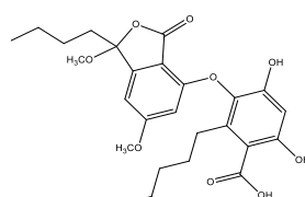
Methyl lobarin
