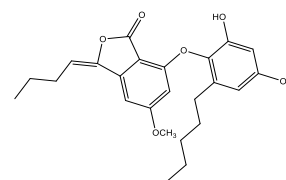
Anhydrosakisacaulon
