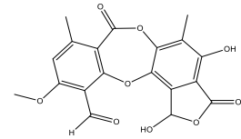
Stictic acid
