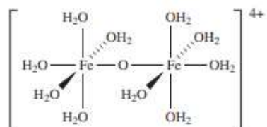
Slika 13. Struktura [(\text{H}_2\text{O})_5\text{FeOFe}(\text{H}_2\text{O})_5]^{4+} .
