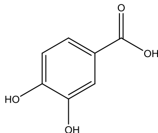
protokatehinska kiselina
