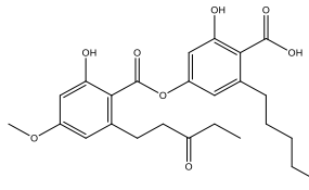
Miriquidic acid
