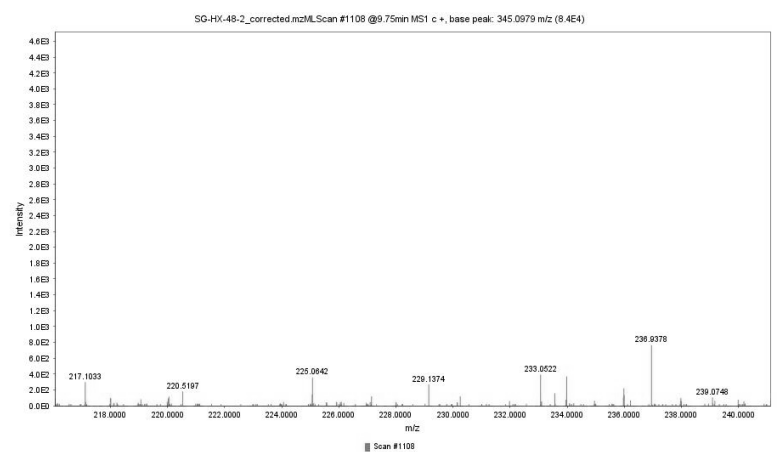
Figure S16. Mass spectrum of ethyl-haematommate with m/z 225.0642.
