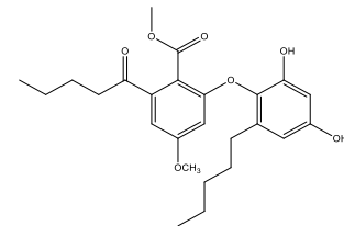
Esterified lobarin
