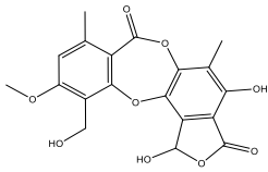
Cryptostictic acid
